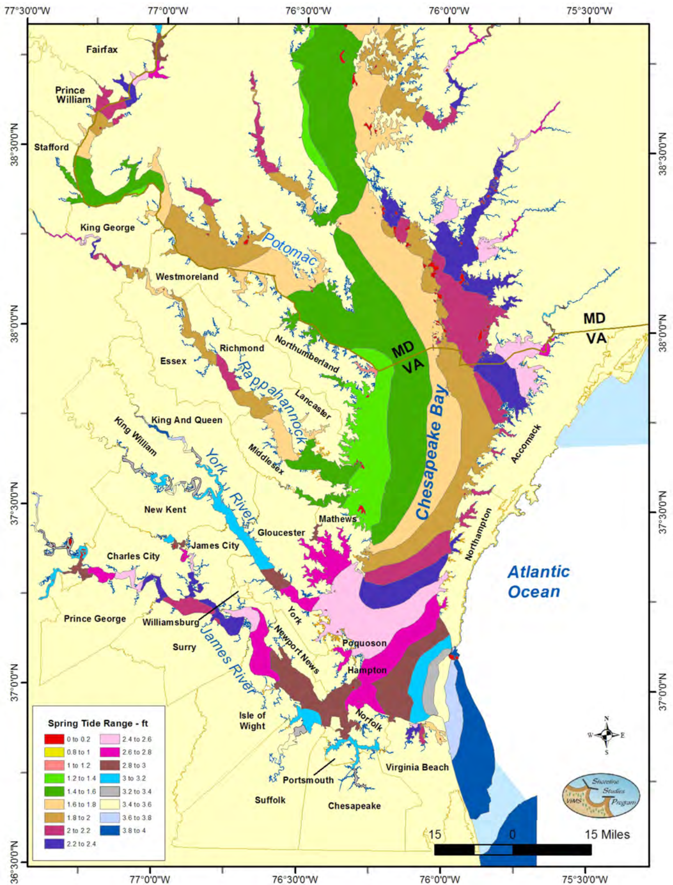
Figure 1-4. Great diurnal (spring) tide ranges in Chesapeake Bay. Tide range polygons interpolated in ArcGIS from data points obtained from NOAA Tides & Currents online. A Google Earth map is available at www.vims.edu/research/departments/physical/programs/ssp/shoreline_management/living_shorelines/class_info .
