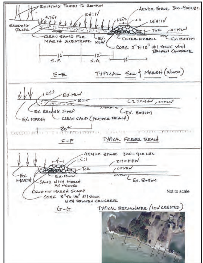
Figure 4-5. Typical cross-sections of the Poplar Grove shore protection system including the sill and marsh, feeder beach, and breakwater. Permit drawings by Coastal Design & Construction, Inc.
