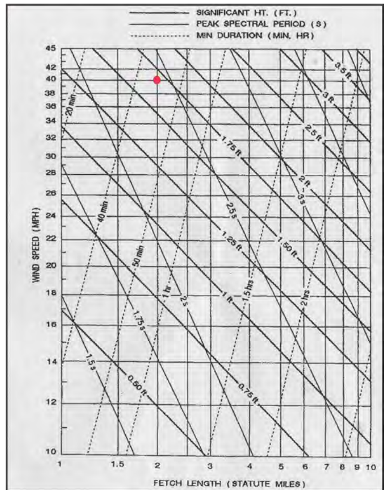
Figure 2-8. Wave height and period estimation using wind speed, duration, and fetch. Appendix 13B-1 from VDOT (2017).
