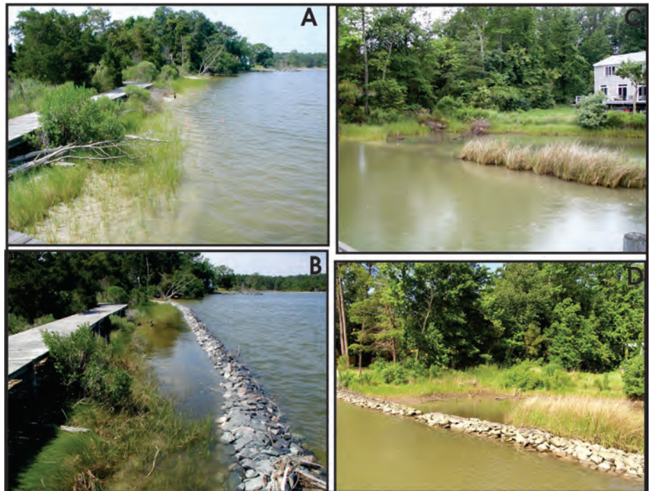
Figure 3-5. Photos showing marsh toe revetments A) before and B) after a project on Cranes Creek in Northumberland County and C) before and D) after a project on Mosquito Creek in Lancaster County, Virginia.
