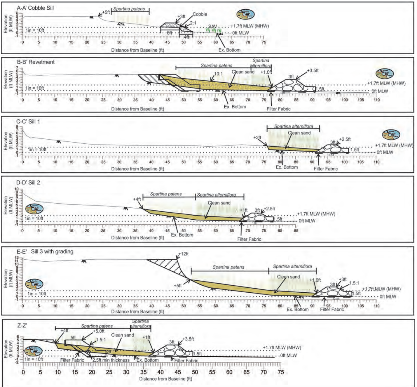
Figure 5-4. Typical cross-section of shore protection structures proposed at Occohannock on the Bay.
