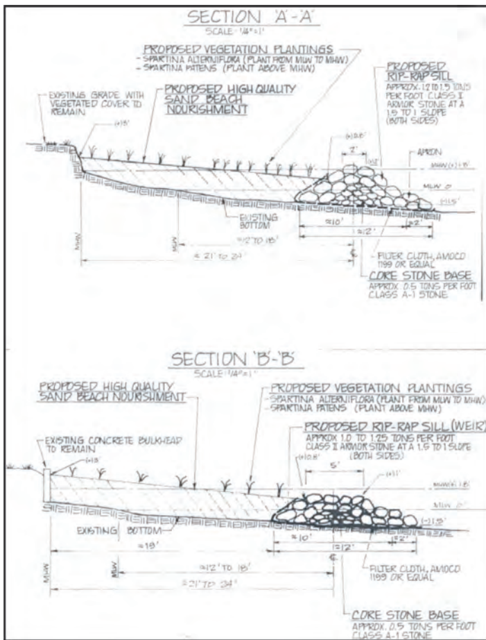
Figure 4-8. Typical cross-sections for sill built at Hull Springs Farm. Section locations are shown on Figure 4-6B. Permit drawings by Bayshore Design, LLC.
