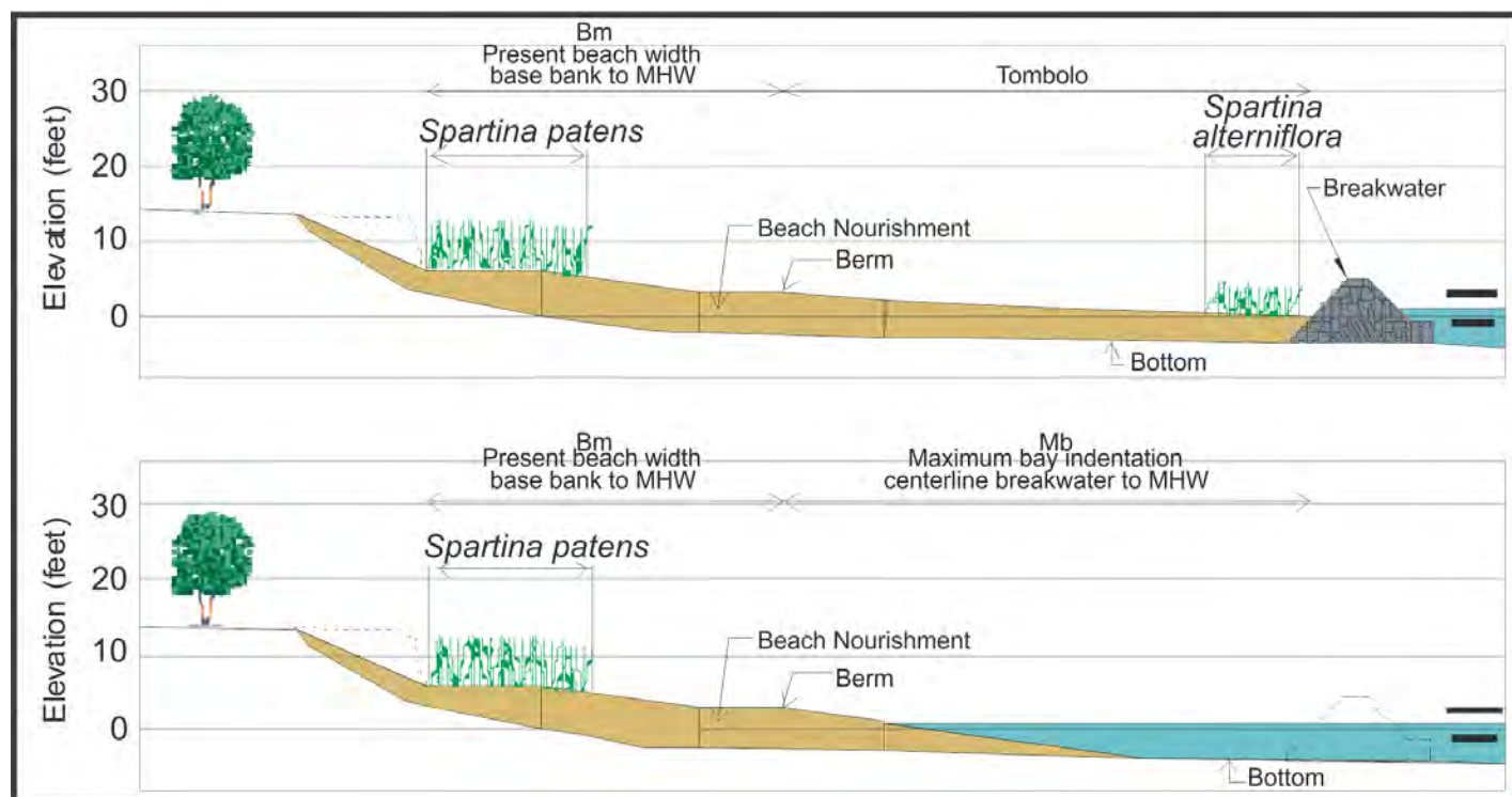
Figure 3-8. Typical tombolo with breakwater and bay beach cross sections (after Hardaway and Byrne, 1999).
