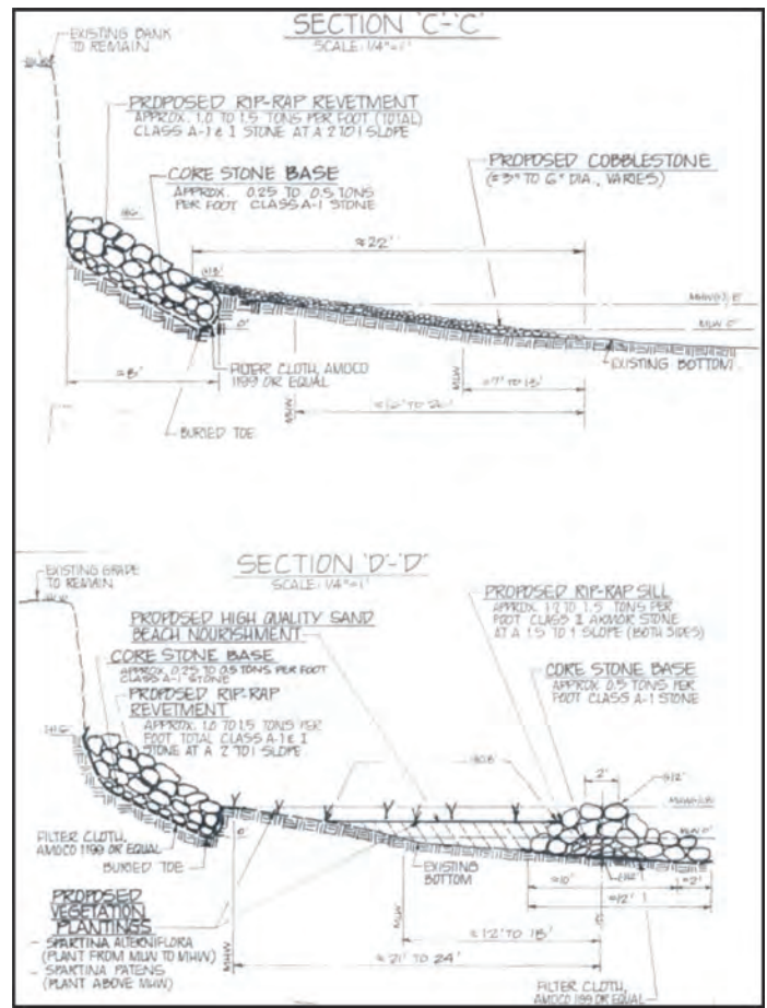
Figure 4-9. Typical cross-sections for sill built at Hull Springs Farm. Section locations are shown on Figure 4-6B. Permit drawings by Bayshore Design, LLC.
