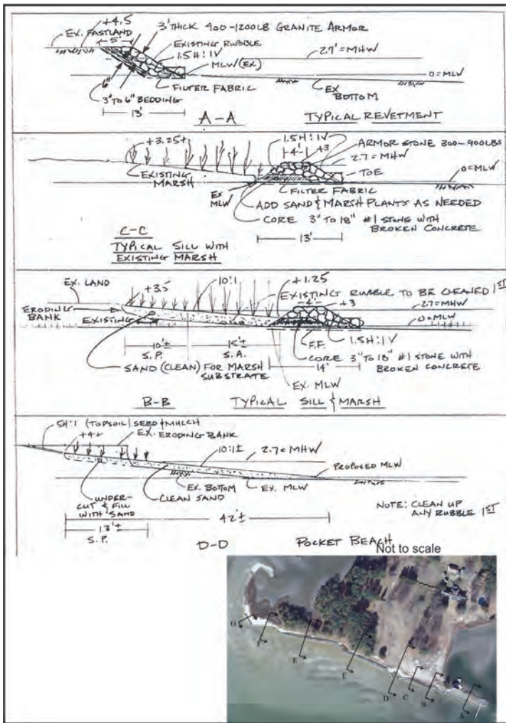
Figure 4-4. Typical cross-sections of the Poplar Grove shore protection system including the revetment, sill and marsh and pocket beach. Permit drawings by Coastal Design & Construction, Inc.
