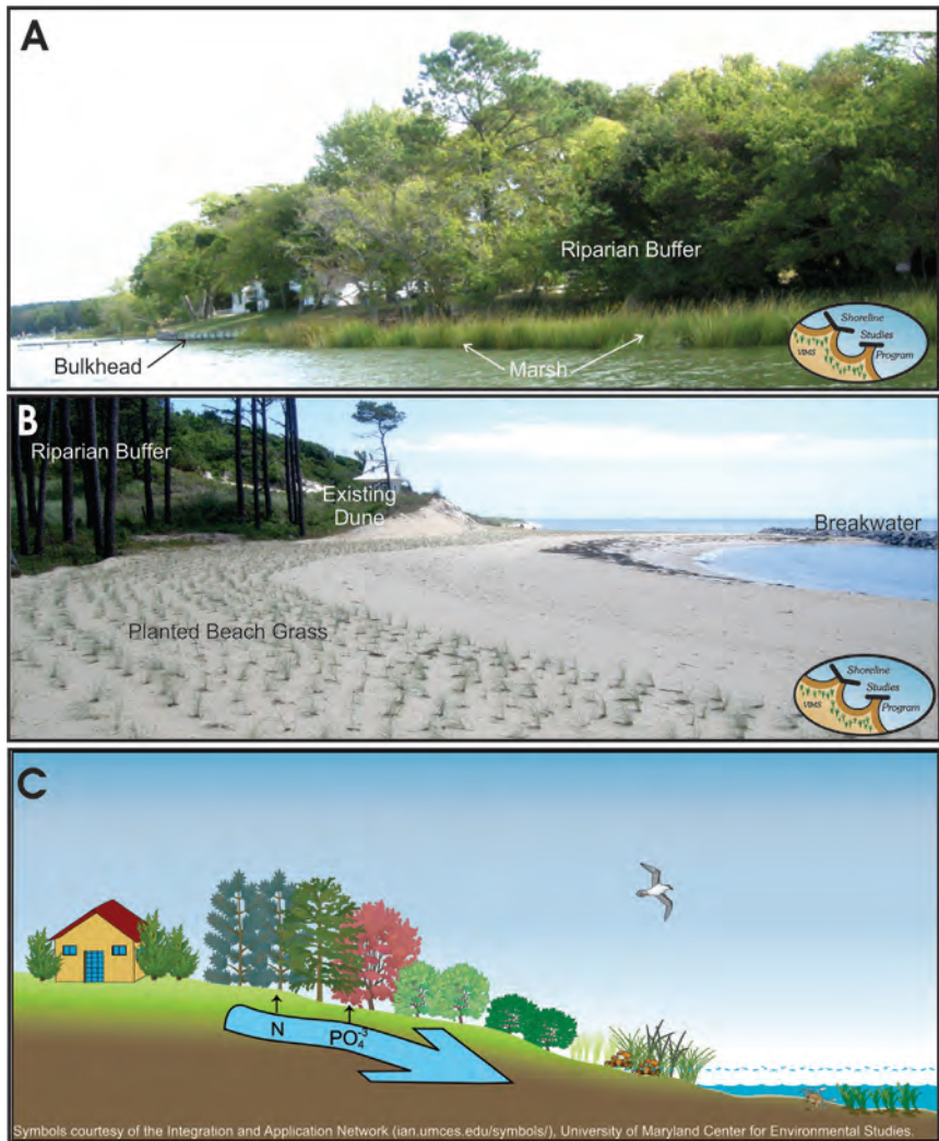
Figure 2-11. Photos depicting aspects of the coastal profile for A) a low-medium energy marsh shoreline and B) a high energy beach shoreline. C) diagram of a connected shore zone shows different landscape elements. C is reprinted courtesy of the University of Maryland Center for Environmental Studies N = Nitrogen, PO4-3 = Phosphate.
