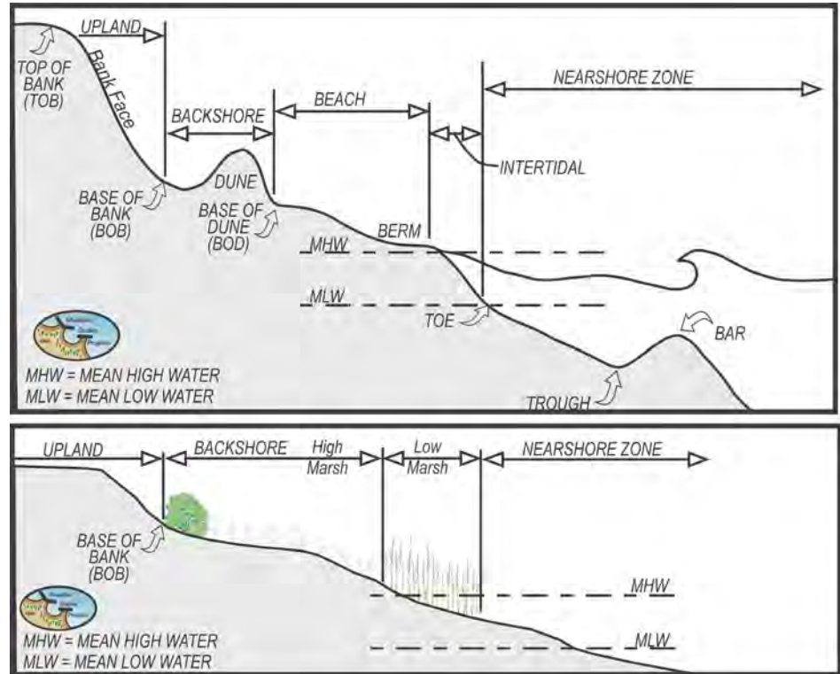
Figure 2-10. Terminology used to identify sections of the shore and backshore zones.
