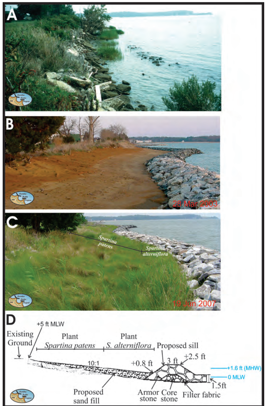
Figure 3-3. Sand fill with stone sills and marsh plantings at Webster Field Annex, St. Mary's County, Maryland A) before installation, B) after installation but before planting, C) after four years, and D) the cross-section used for construction (Hardaway et al. , 2009).
