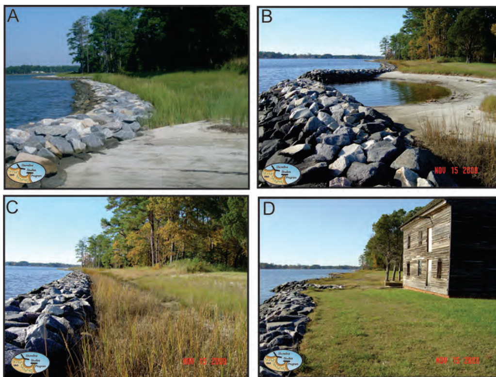
Figure 4-3. Sill system at Poplar Grove on the East River in Mathews County, Virginia six years after completion. A) The sill and marsh fringe provide a wide buffer between the water and the upland. B) The wide gap in the sill provides a pocket beach access area along the shoreline. C) The project zones are clearly visible: stone sill, S. alterniflora , S. patens , and upland/wooded. D) The old mill sits close to the shoreline. In this area, a revetment was chosen to protect the shoreline.
