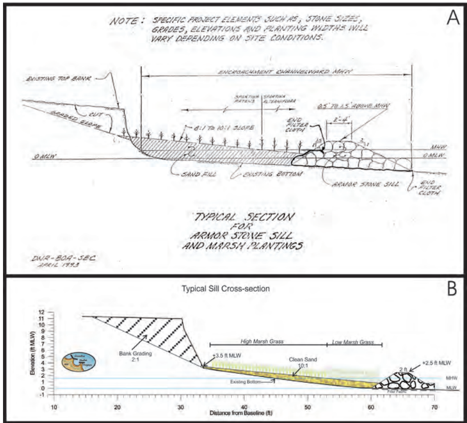
Figure 3-4. Typical sill cross-section A) created by Maryland Department of Natural Resources for their non-structural program and B) designed for Robin Grove Park in Colonial Beach. The mean tide range is 1.6 ft, so mid-tide level is 0.8 ft MLW. The level of protection in this case is +3.5 ft MLW, so the sand fill should be graded on an 10:1 slope from the bank to the back of the sill. The upland bank should also be graded and re-vegetated.
