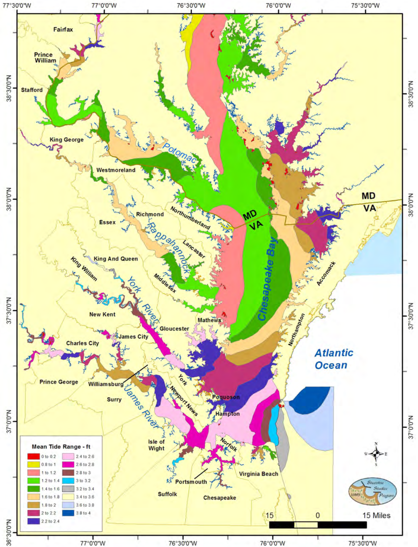
Figure 1-3. Mean tide ranges in Chesapeake Bay. Tide range polygons interpolated in ArcGIS from data points obtained from NOAA Tides & Currents online. A Google Earth map is available at www.vims.edu/research/departments/physical/programs/ssp/shoreline_management/living_shorelines/class_info .
