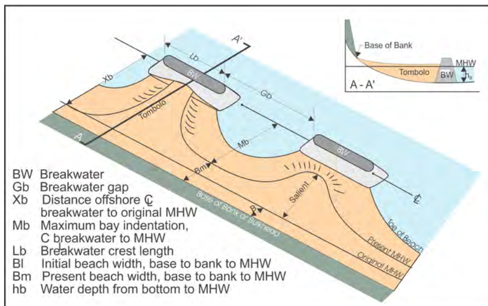
Figure 3-7. Breakwater design parameters (after Hardaway and Byrne, 1999).
