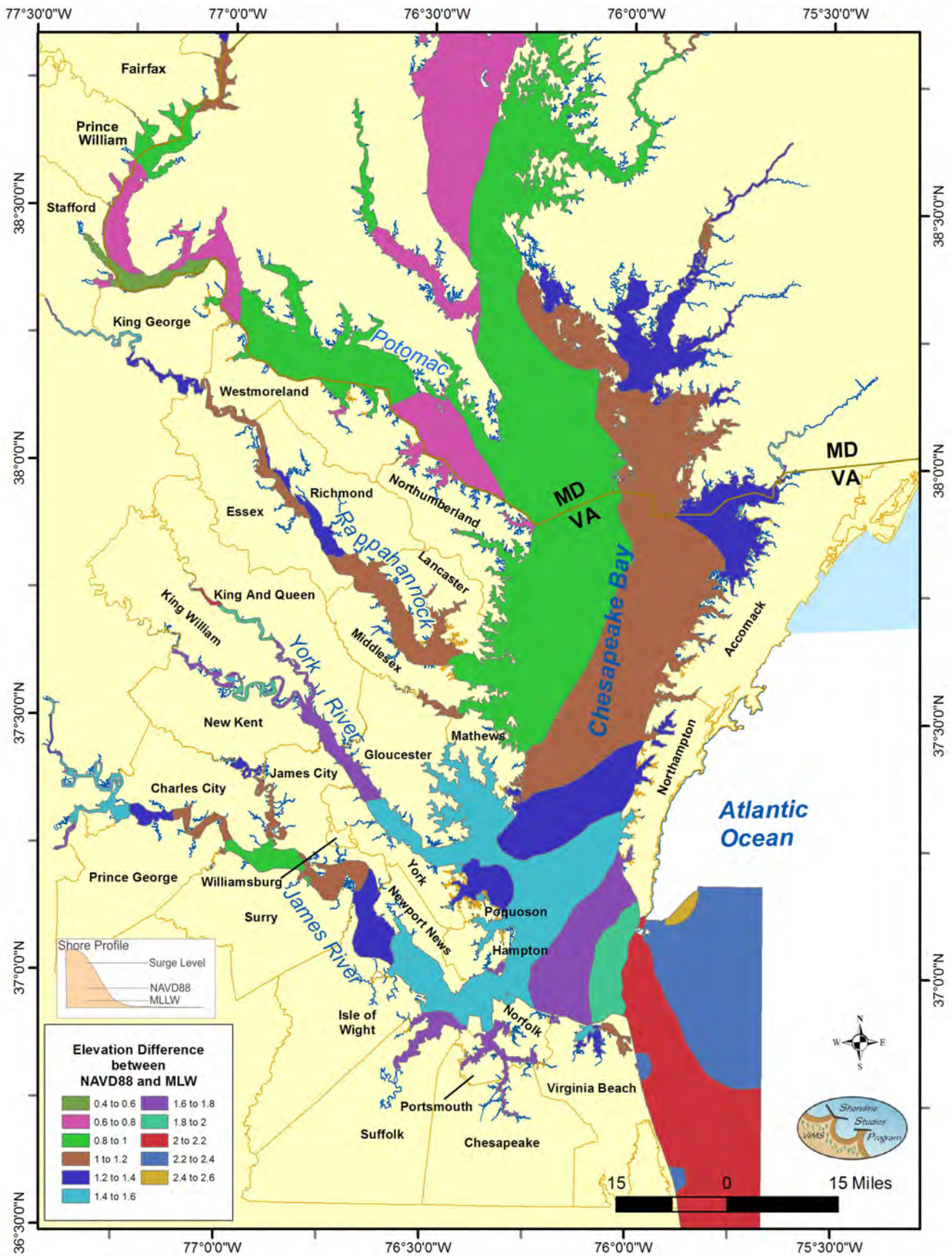
Figure 2-6. Map depicting the elevation difference between NAVD88 and MLLW in Chesapeake Bay. Data calculated using NOAA's VDATUM grids. Datum transformation grid TSS was subtracted from the MLLW datum transformation grid ( http://vdatum.noaa.gov/dev/gtx_info.html ) to obtain the elevation differences. A Google Earth application is available at www.vims.edu/research/departments/physical/programs/ssp/shoreline_management/living_shorelines/class_info .
